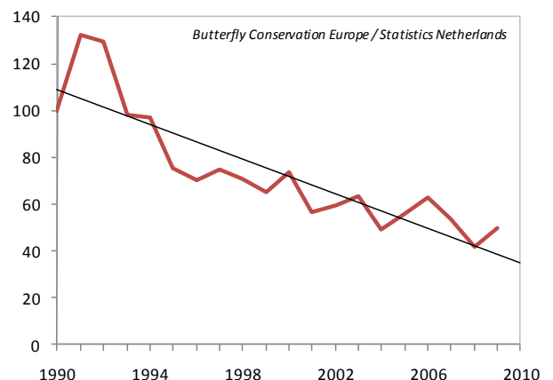
The European Grassland Butterfly Indicator shows a dramatic decline of almost 70%.
